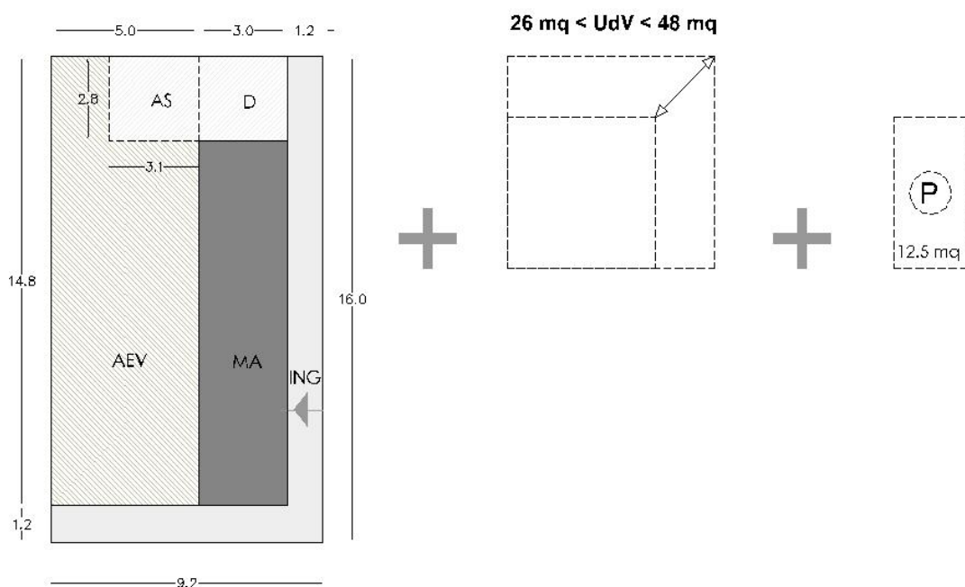
Fig. 1 - The elements of the Minimal Housing Unit (example of the Module "container" for 3/4 users)
